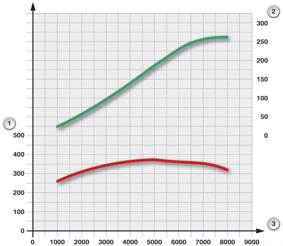
Fig. 30: Torque and power curve
