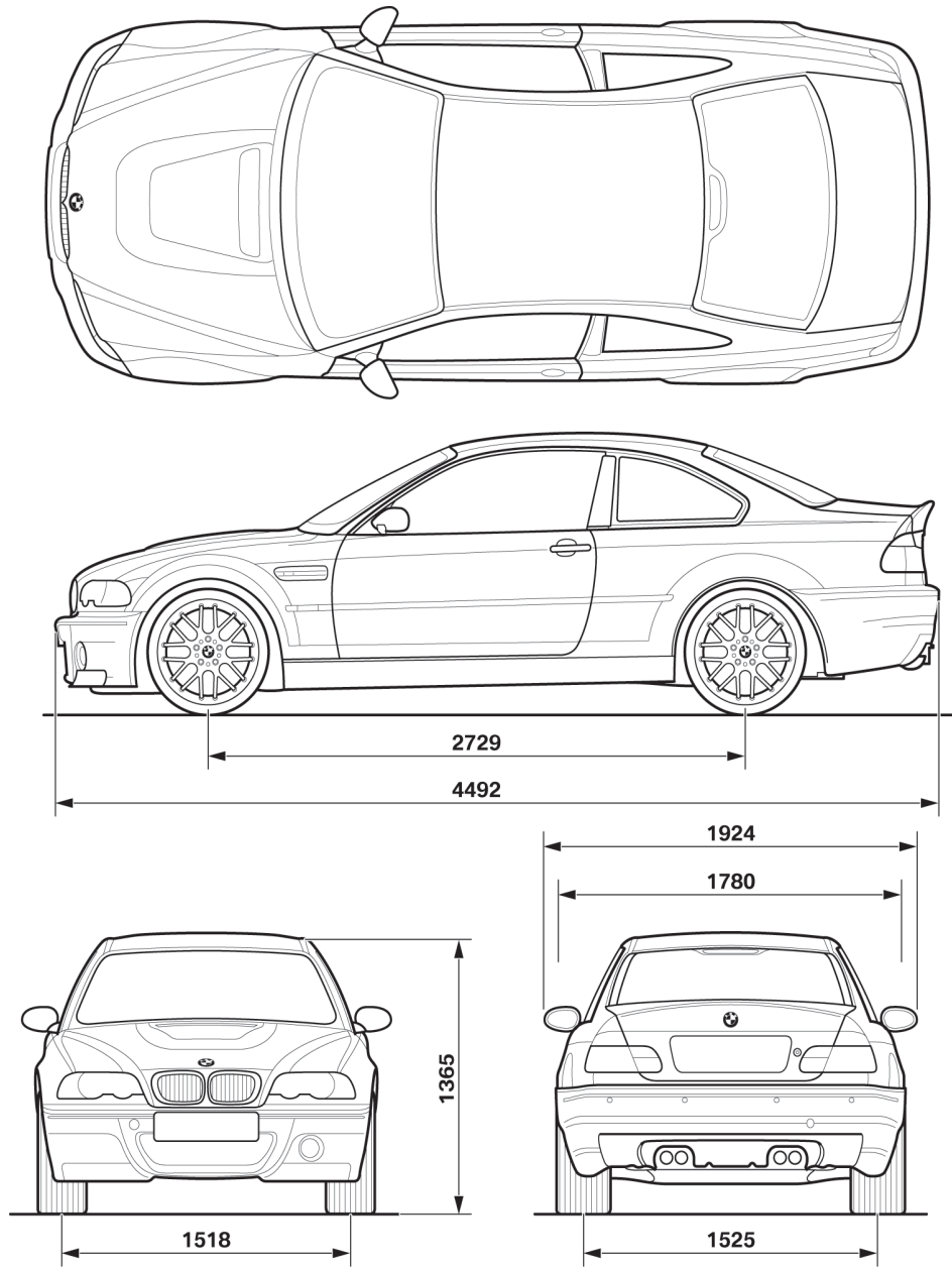
Fig. 7: Vehicle dimensions
